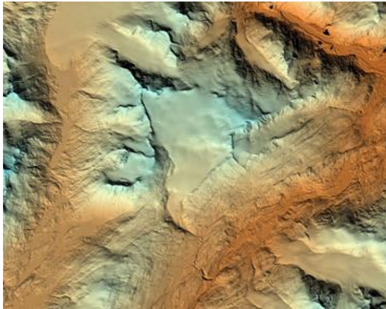
Figure 6: Pan-Arctic DEM
